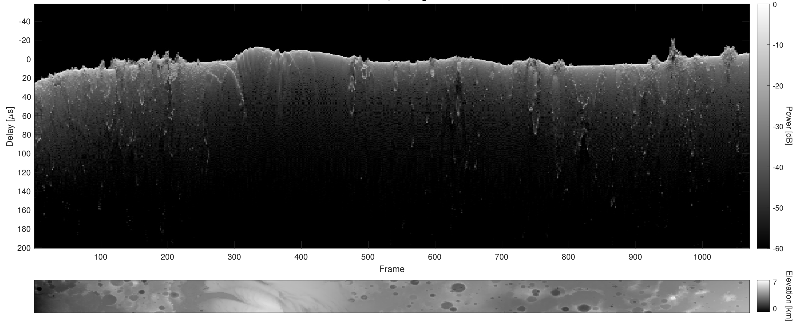
Orbit 12815, Cluttergram
