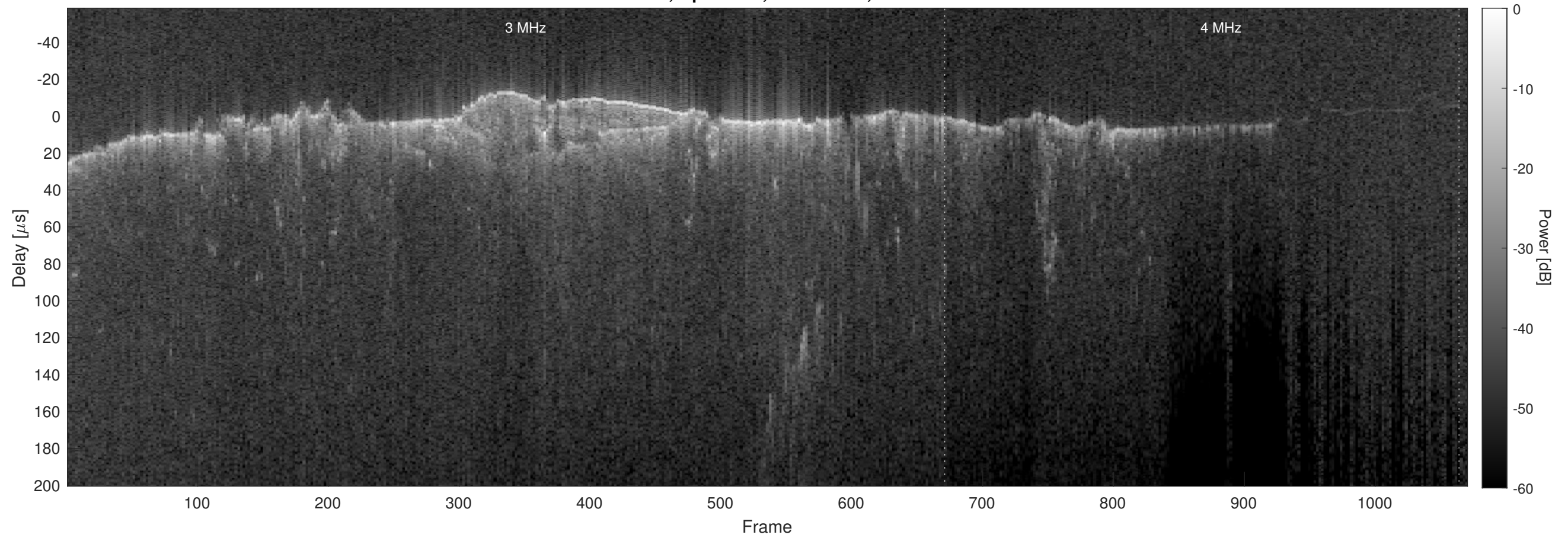
Orbit 12815, Optimized, No Window, Channel 2
