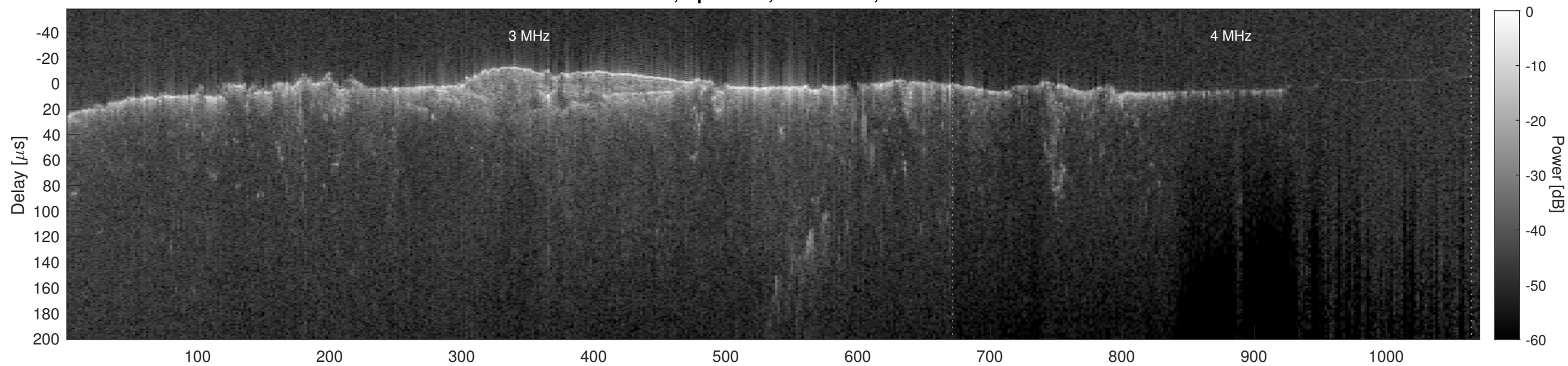
Orbit 12815, Cluttergram
