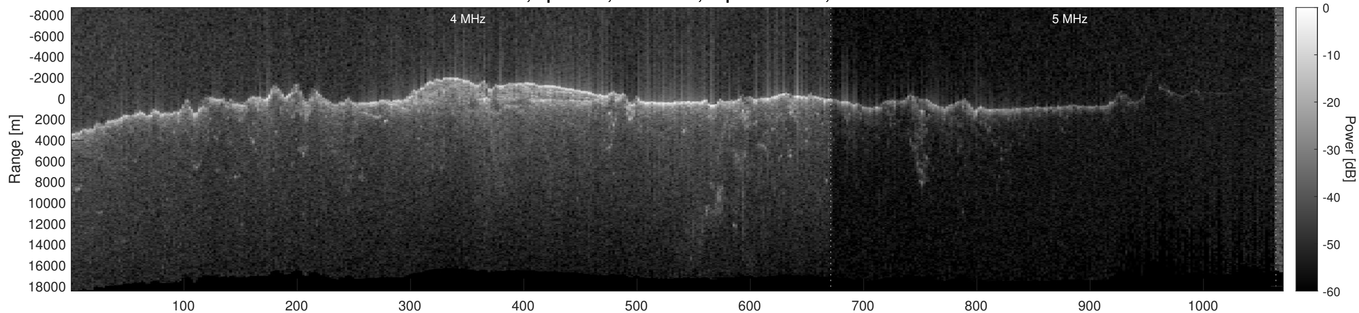
Orbit 12815, Optimized, No Window, Depth-Corrected, Channel 2
