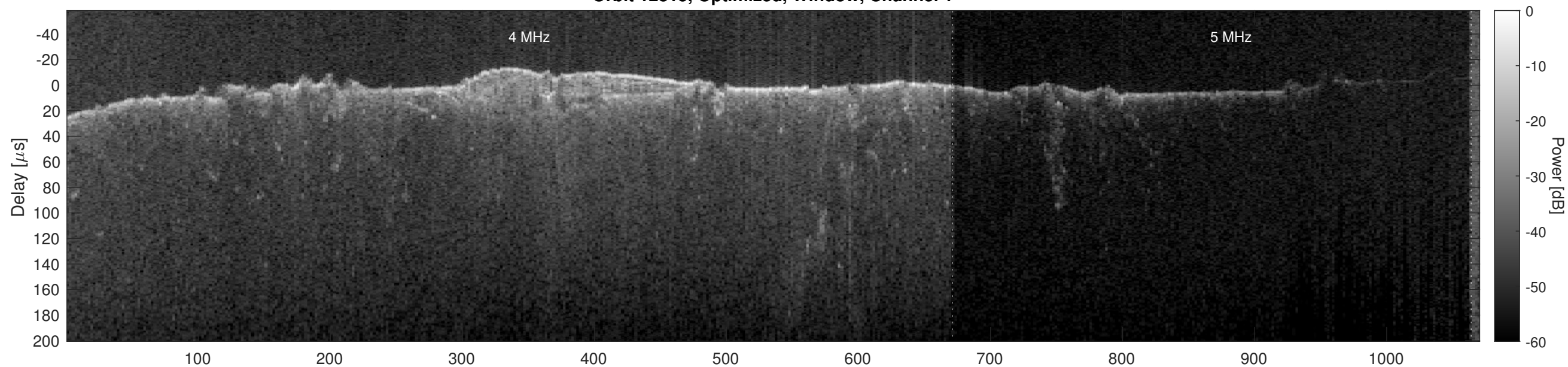
Orbit 12815, Optimized, Window, Channel 2
