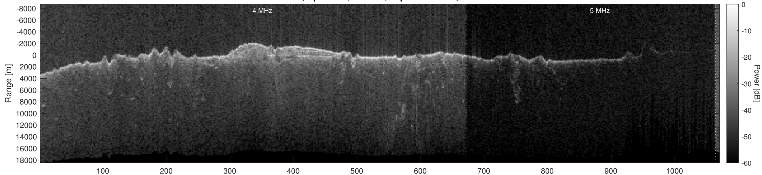
Orbit 12815, Optimized, Window, Depth-Corrected, Channel 2
