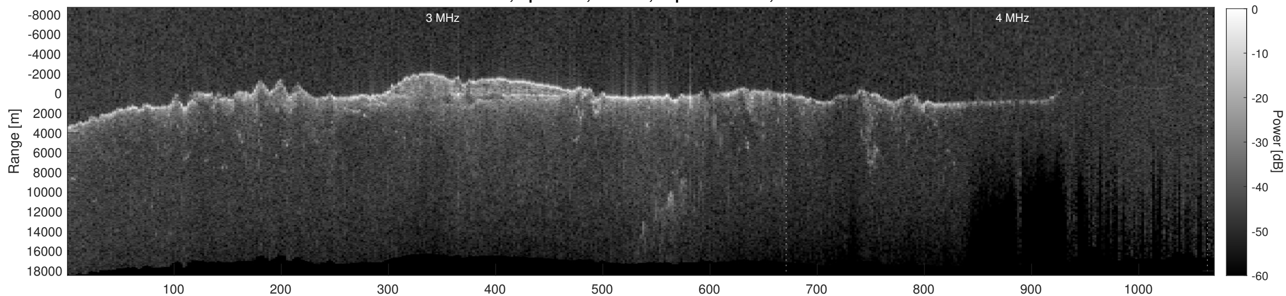
Orbit 12815, Depth-Corrected Cluttergram
