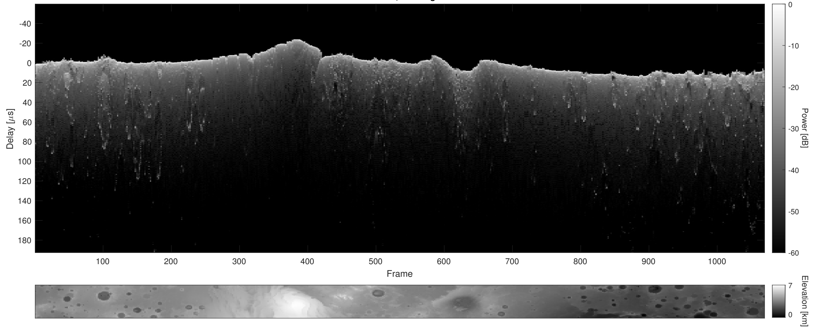
Orbit 12817, Cluttergram
