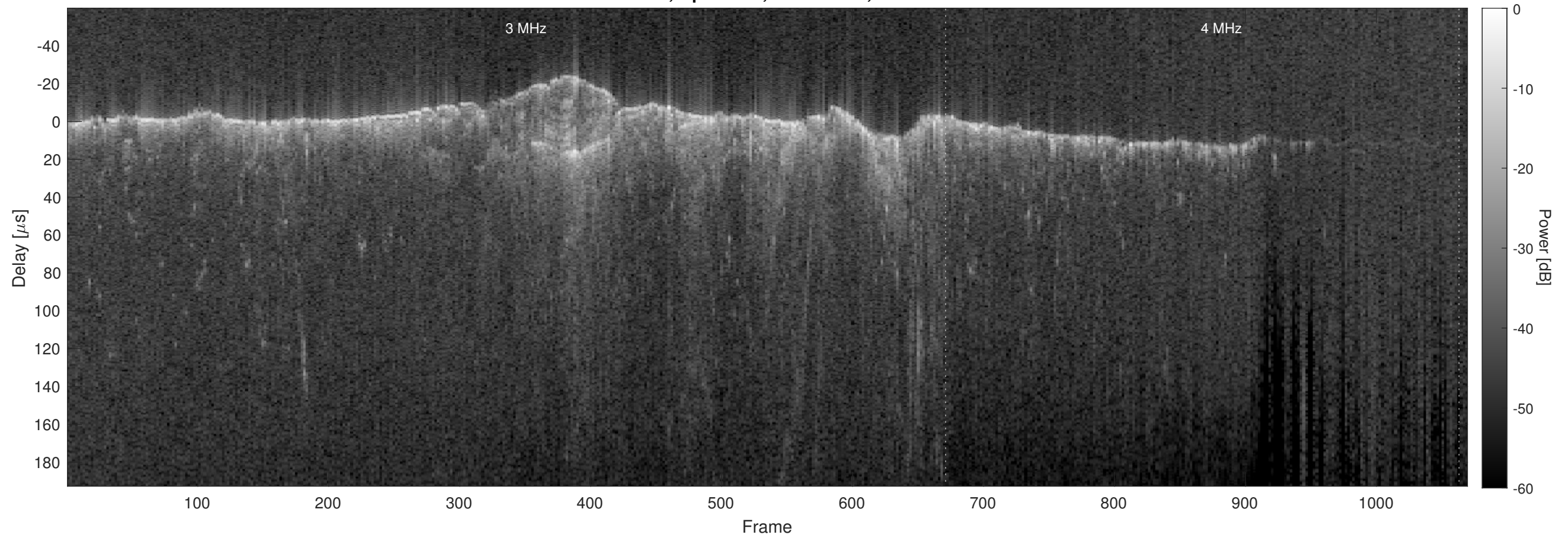
Orbit 12817, Optimized, No Window, Channel 2
