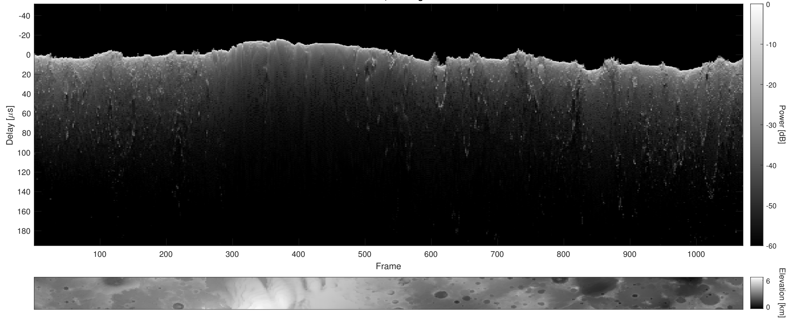
Orbit 12819, Cluttergram
