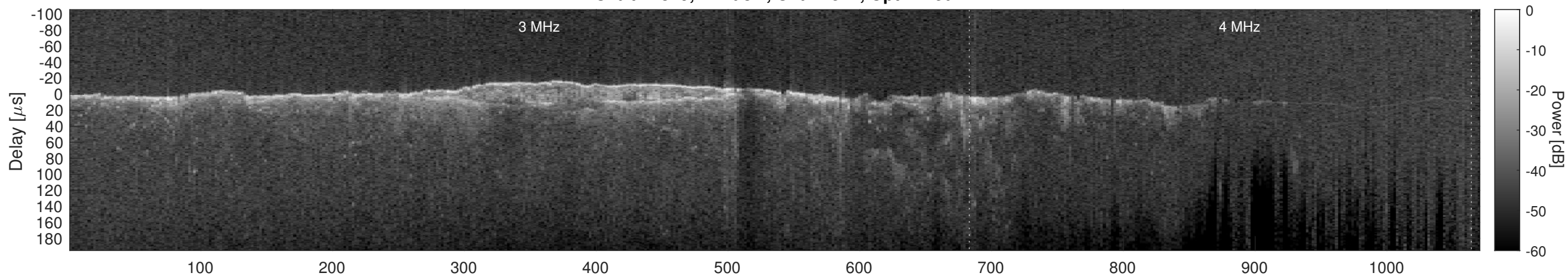
Orbit 12819, Cluttergram
