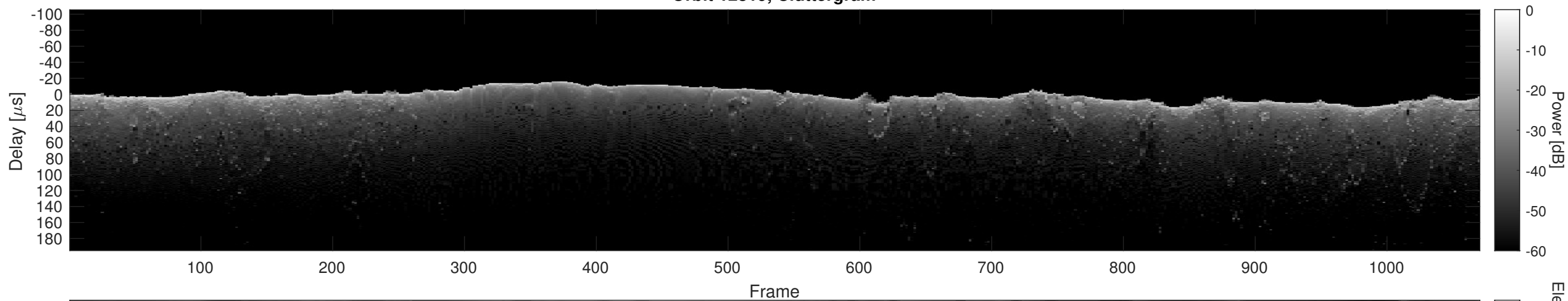
Orbit 12819, Cluttergram
