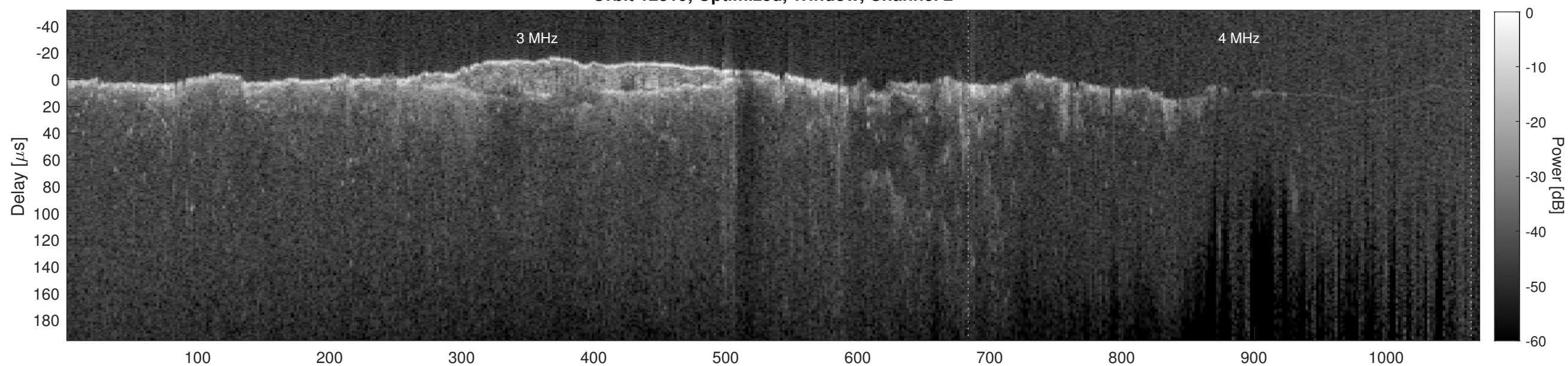
Orbit 12819, Cluttergram
