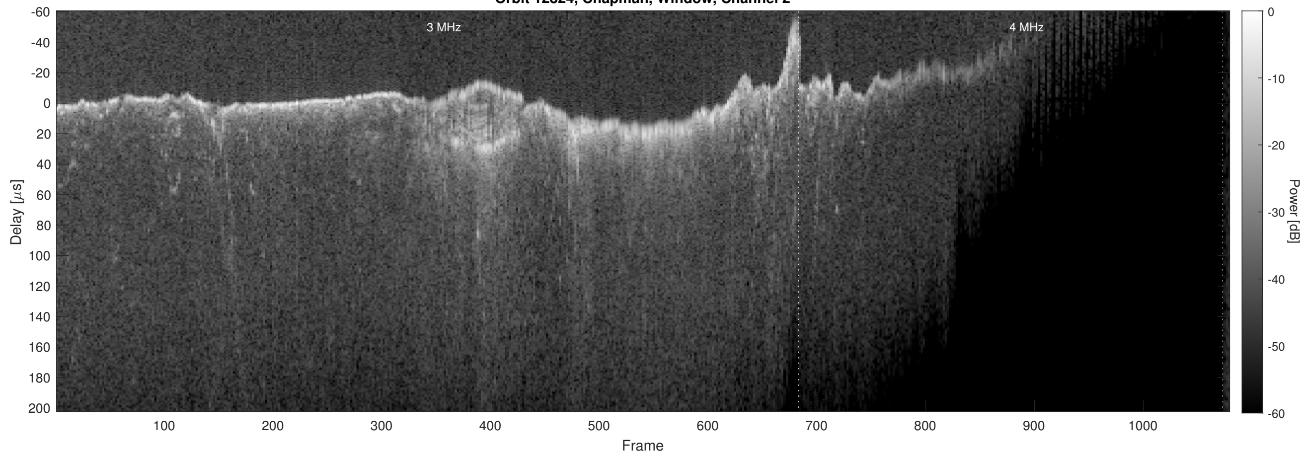
Orbit 12824, Chapman, Window, Channel 2
