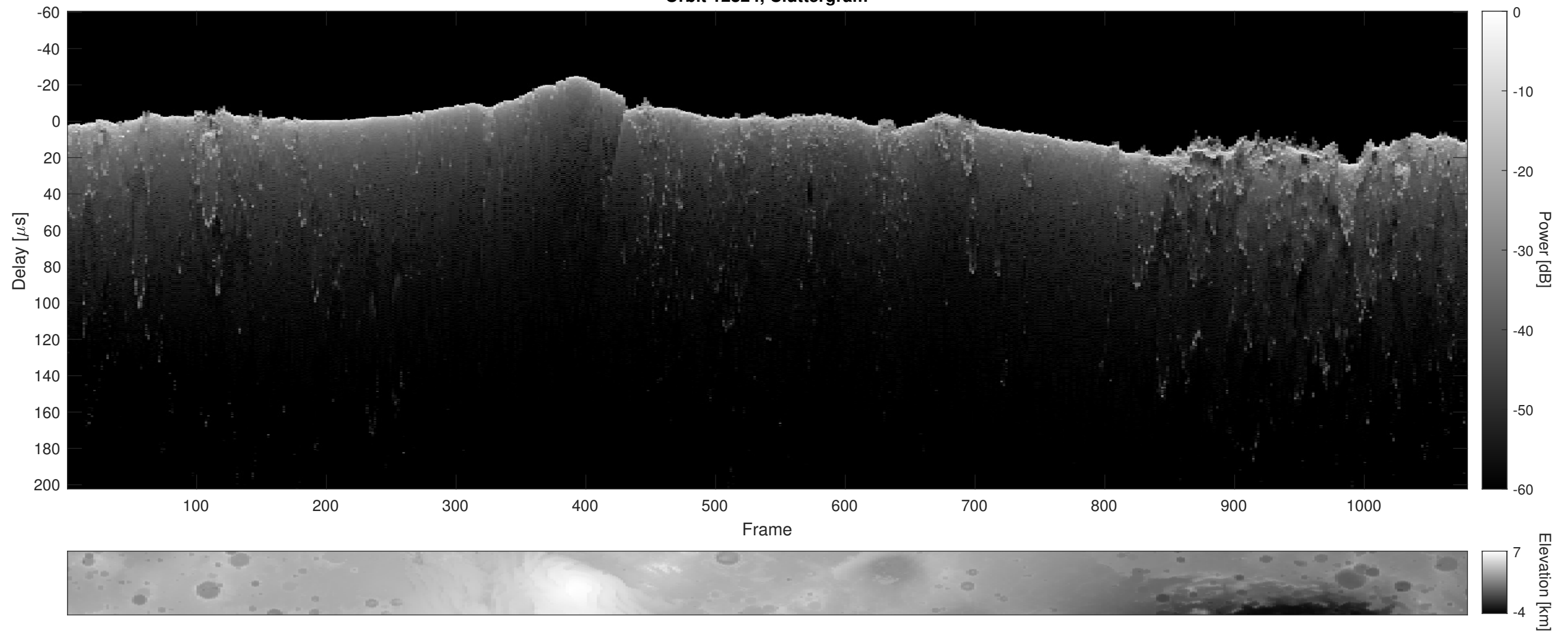
Orbit 12824, Cluttergram
