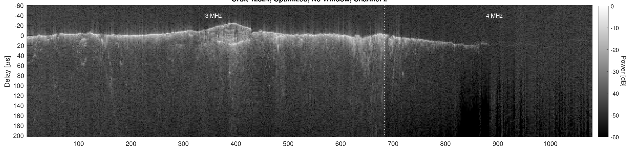
Orbit 12824, Cluttergram
