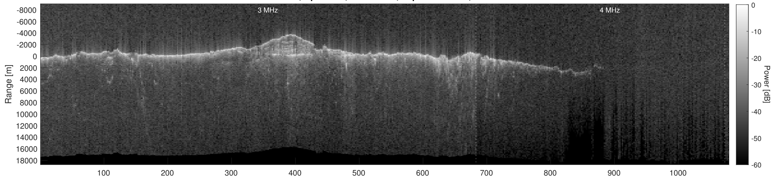
Orbit 12824, Depth-Corrected Cluttergram
