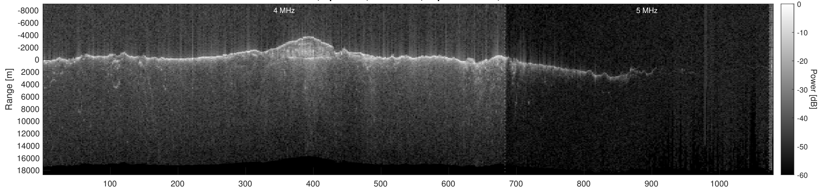
Orbit 12824, Optimized, No Window, Depth-Corrected, Channel 2
