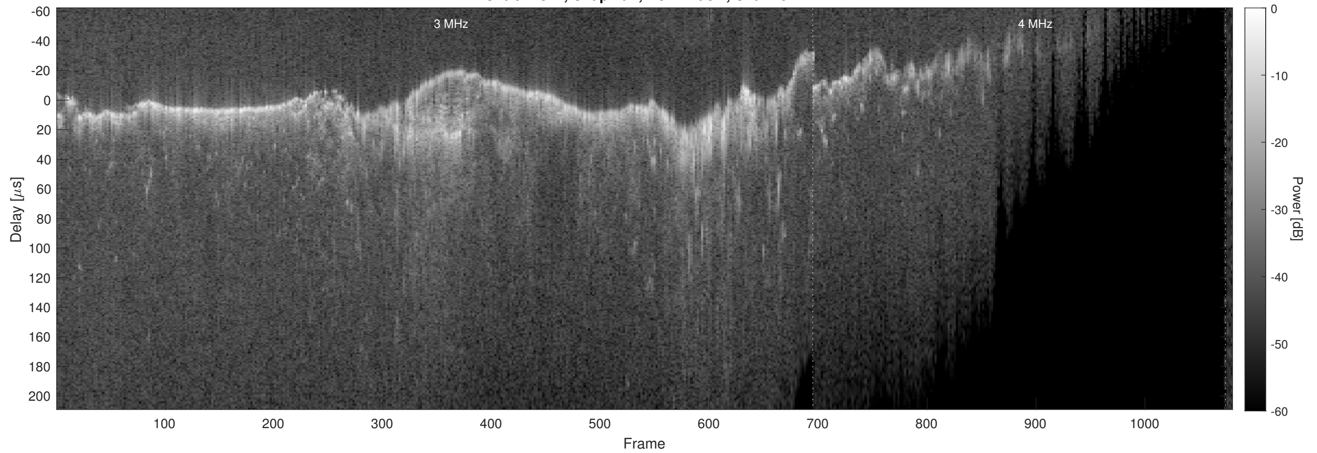
Orbit 12827, Chapman, No Window, Channel 2
