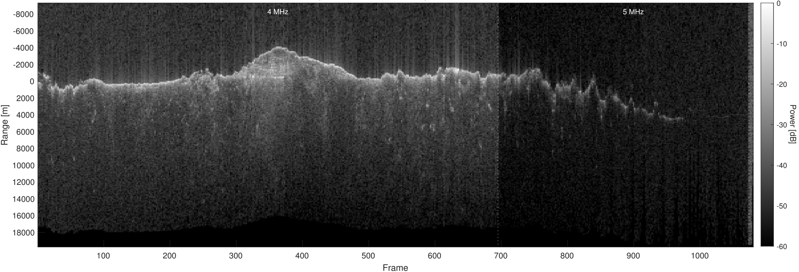
Orbit 12827, Optimized, No Window, Depth-Corrected, Channel 2
