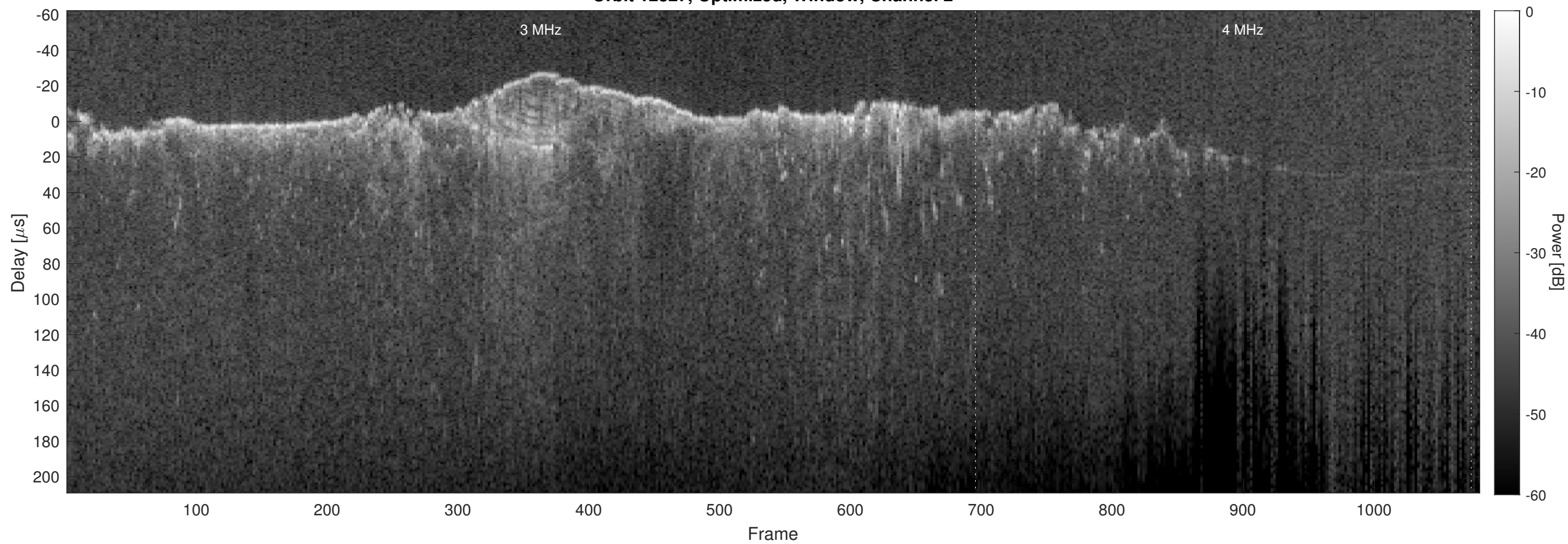
Orbit 12827, Optimized, Window, Channel 2
