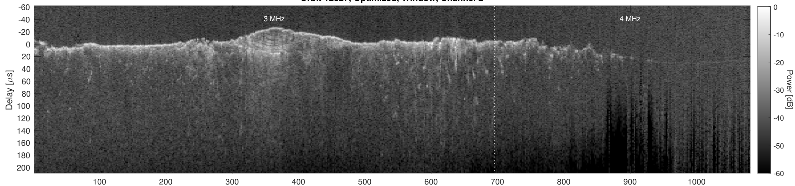
Orbit 12827, Cluttergram
