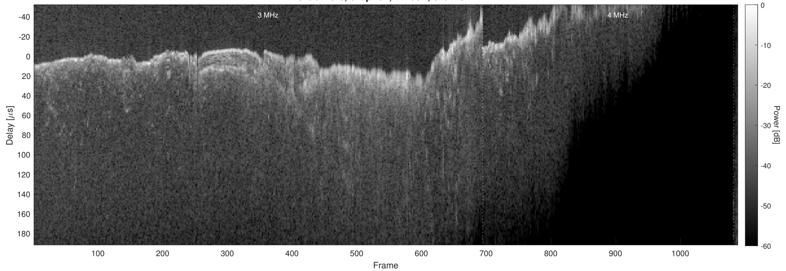
Orbit 12828, Chapman, Window, Channel 2
