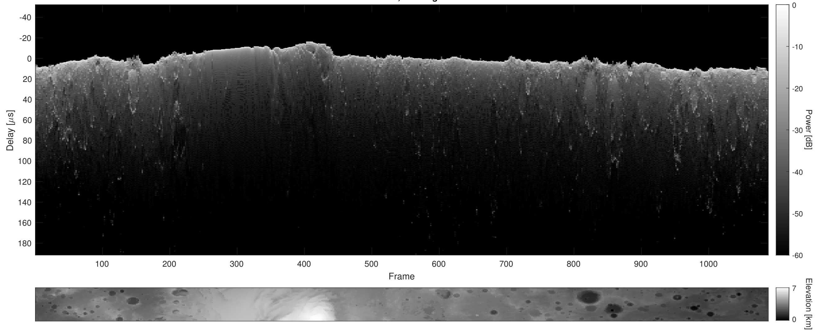
Orbit 12828, Cluttergram
