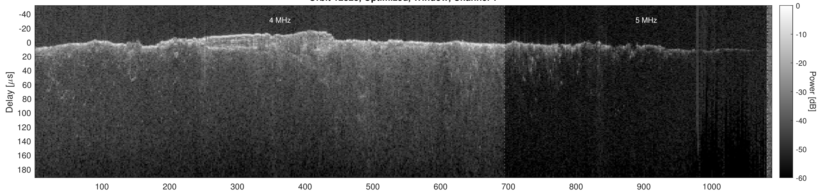
Orbit 12828, Optimized, Window, Channel 2
