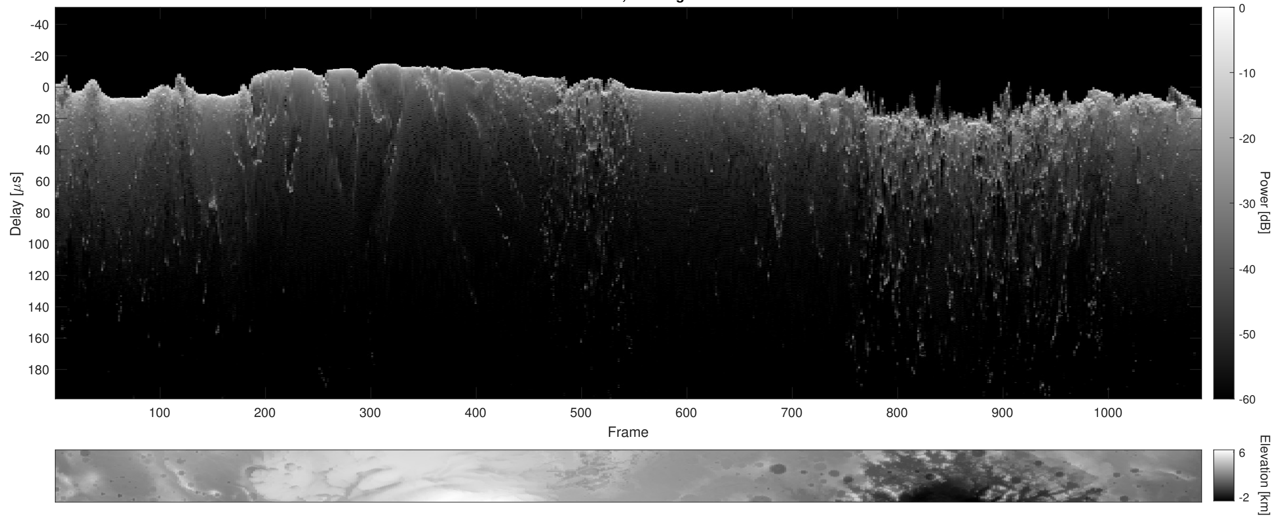
Orbit 12832, Cluttergram
