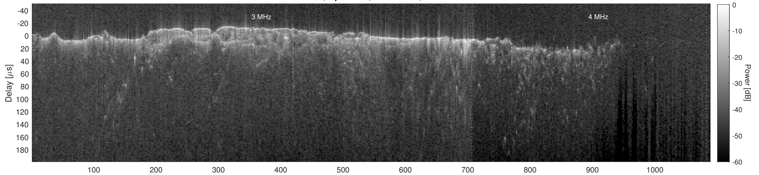
Orbit 12832, Cluttergram
