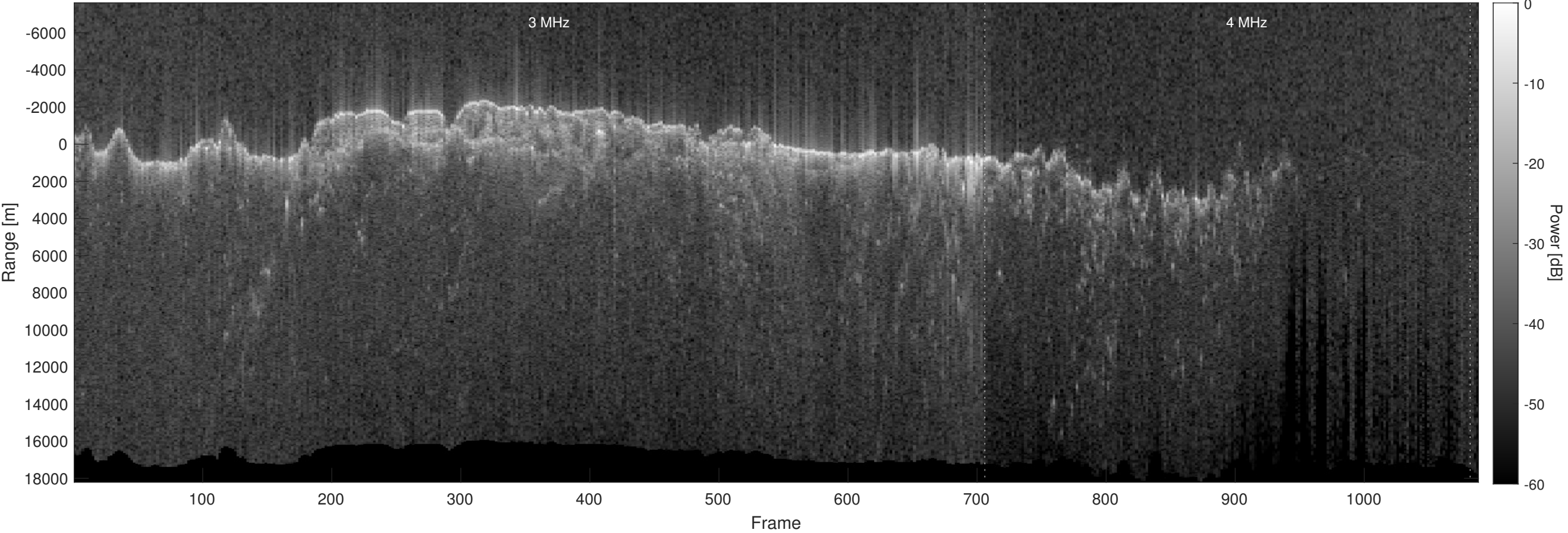
Orbit 12832, Optimized, No Window, Depth-Corrected, Channel 2
