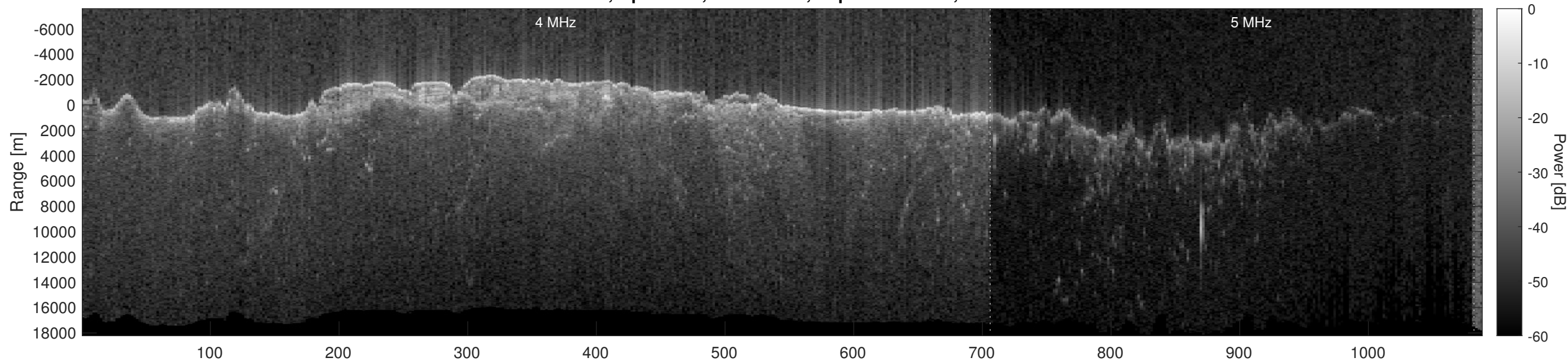
Orbit 12832, Optimized, No Window, Depth-Corrected, Channel 2
