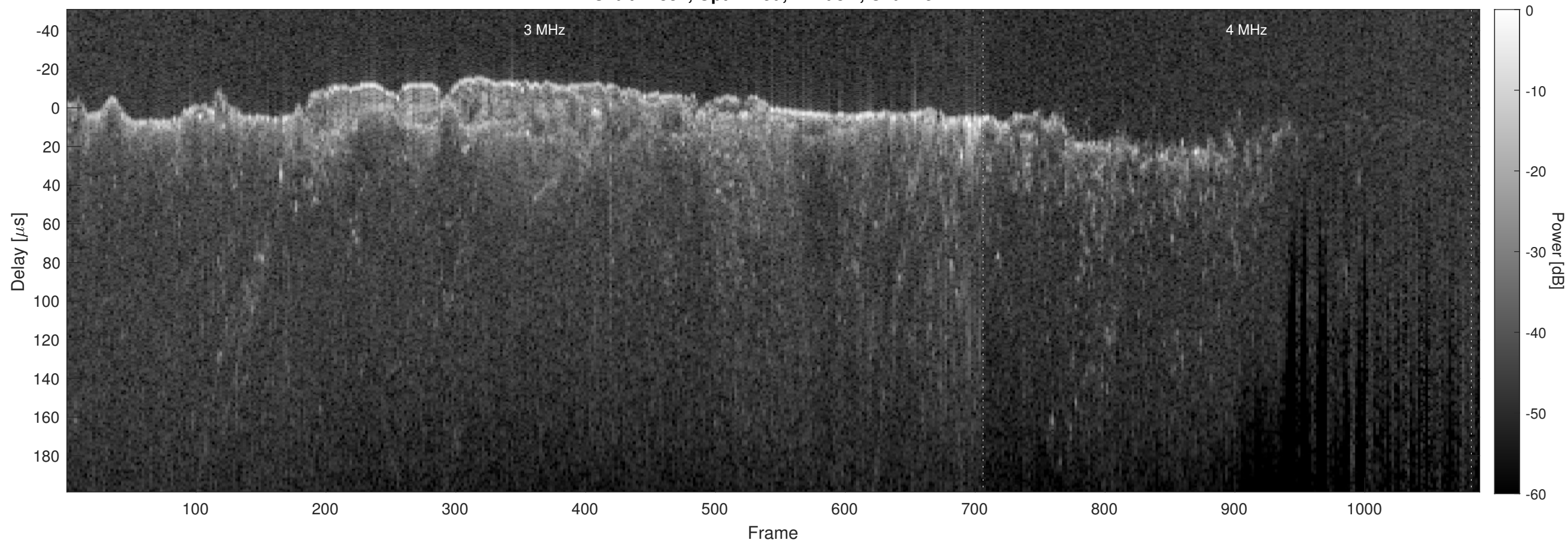
Orbit 12832, Optimized, Window, Channel 2
