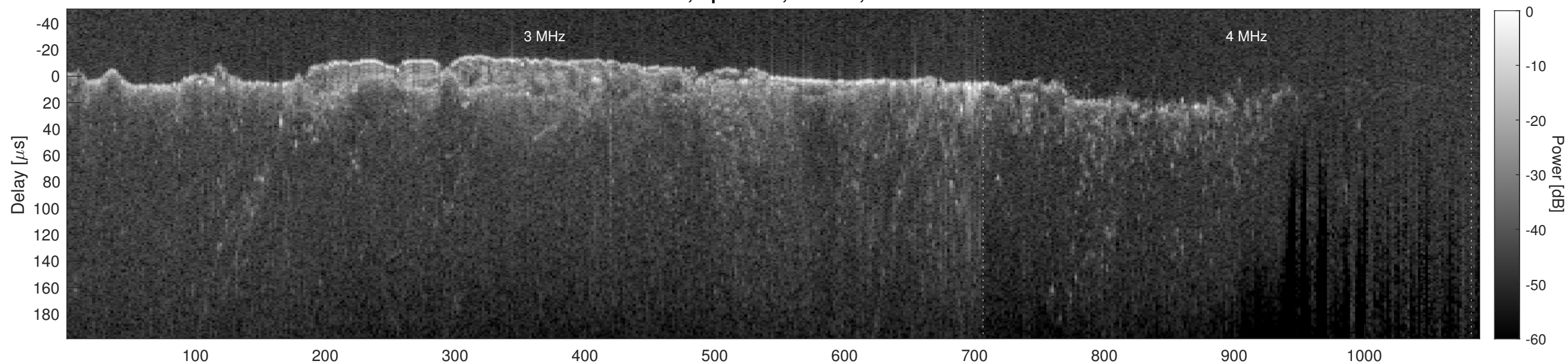
Orbit 12832, Cluttergram
