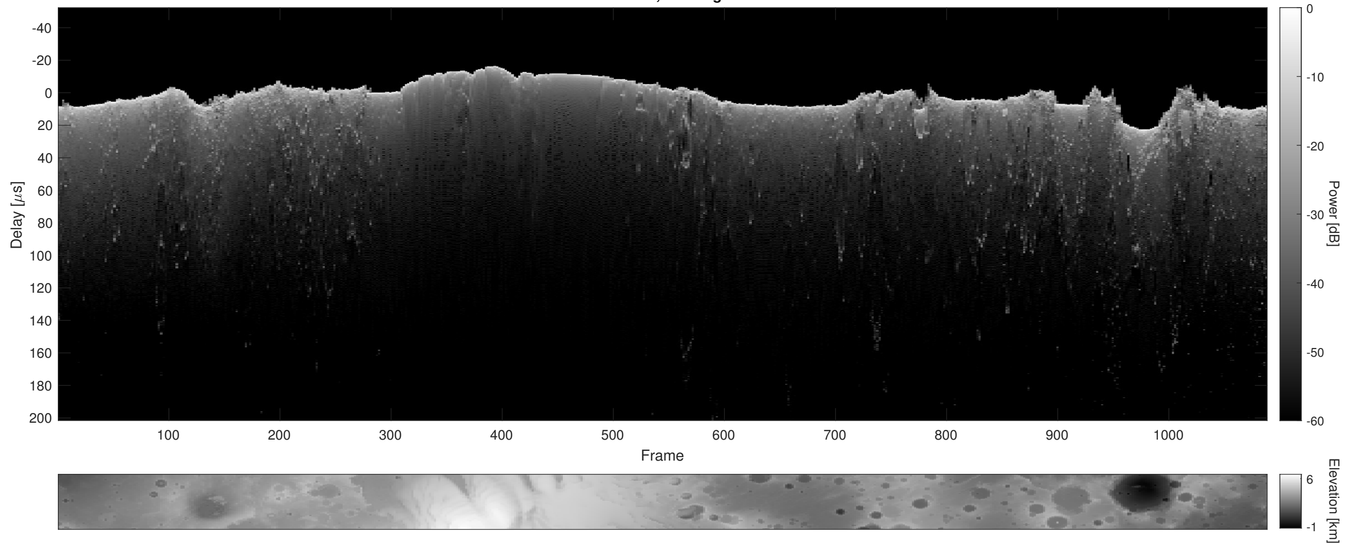
Orbit 12833, Cluttergram
