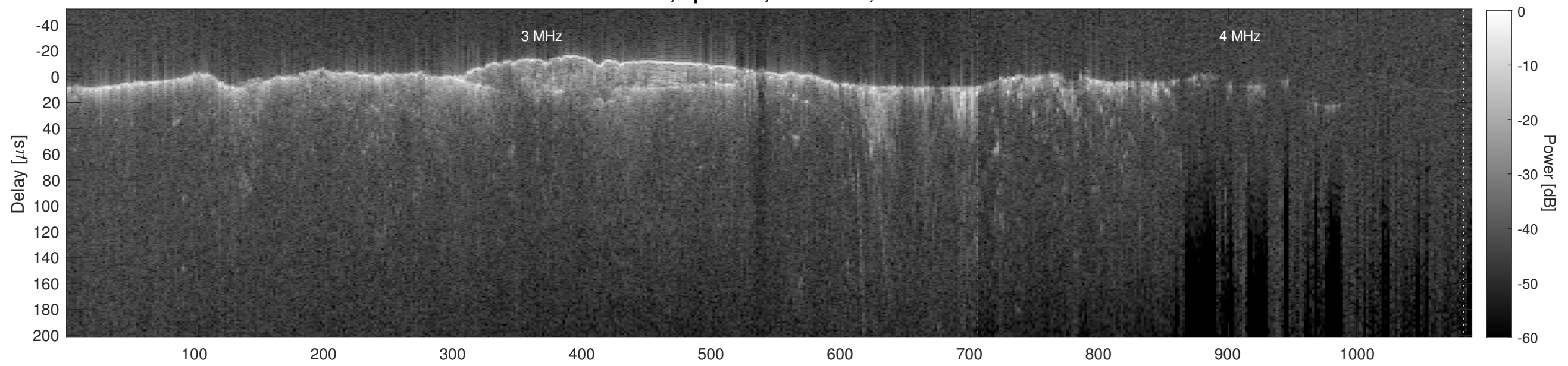
Orbit 12833, Cluttergram
