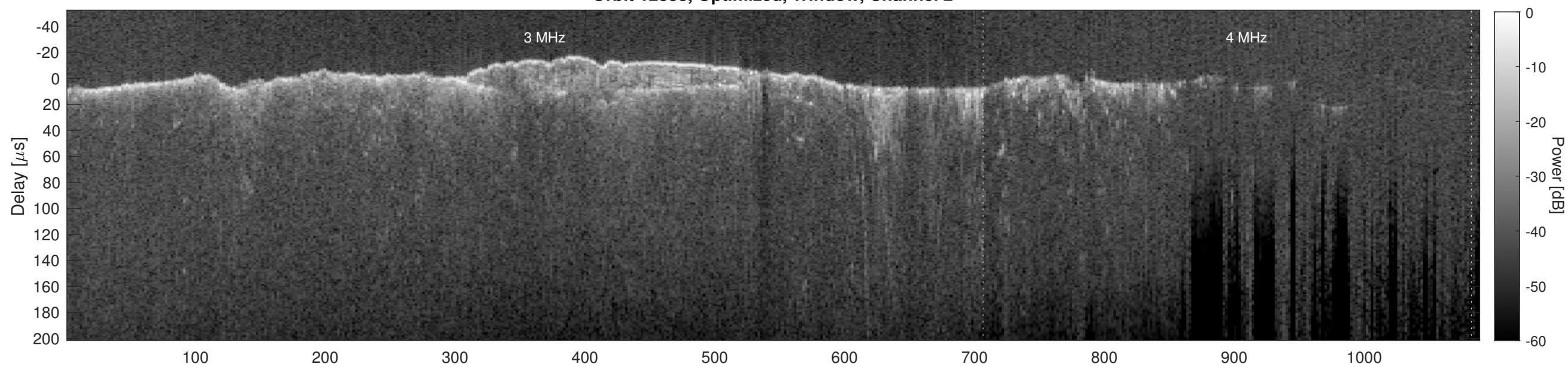
Orbit 12833, Cluttergram
