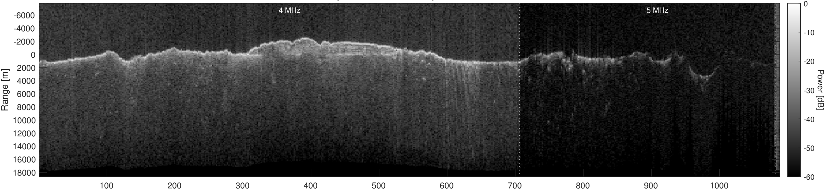
Orbit 12833, Optimized, Window, Depth-Corrected, Channel 2
