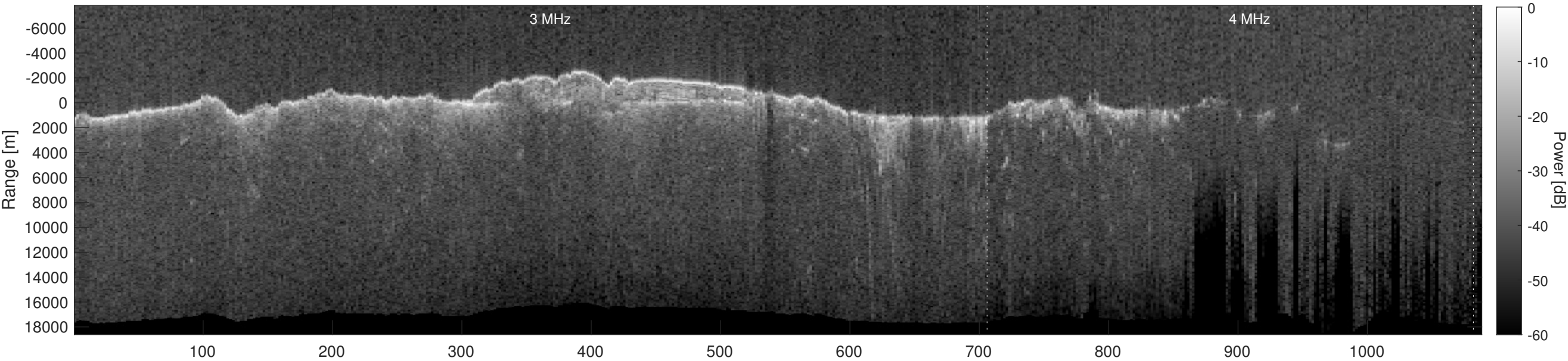
Orbit 12833, Depth-Corrected Cluttergram
