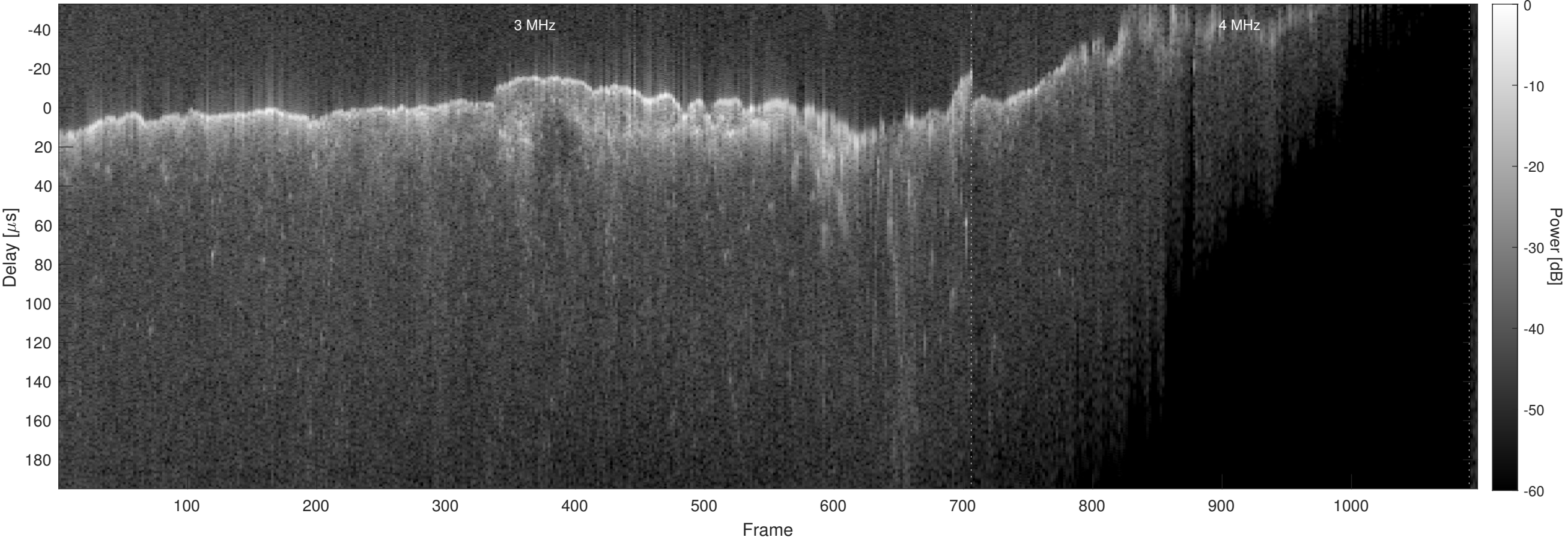
Orbit 12837, Chapman, No Window, Channel 2
