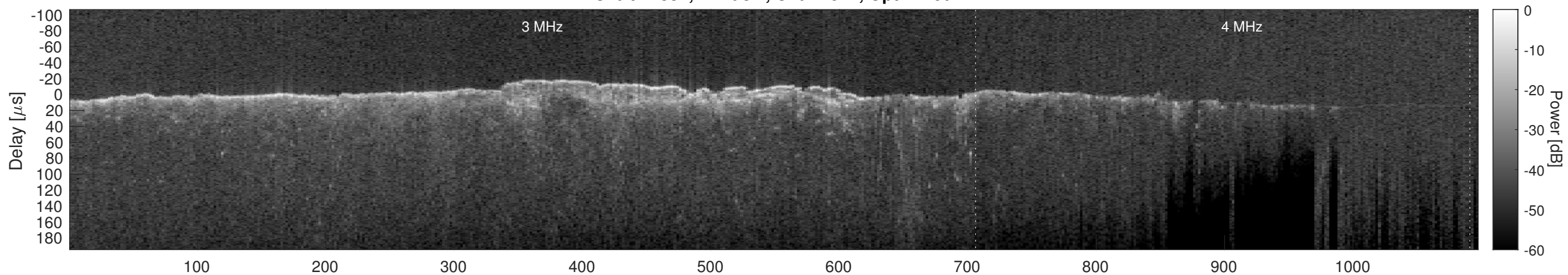
Orbit 12837, Cluttergram
