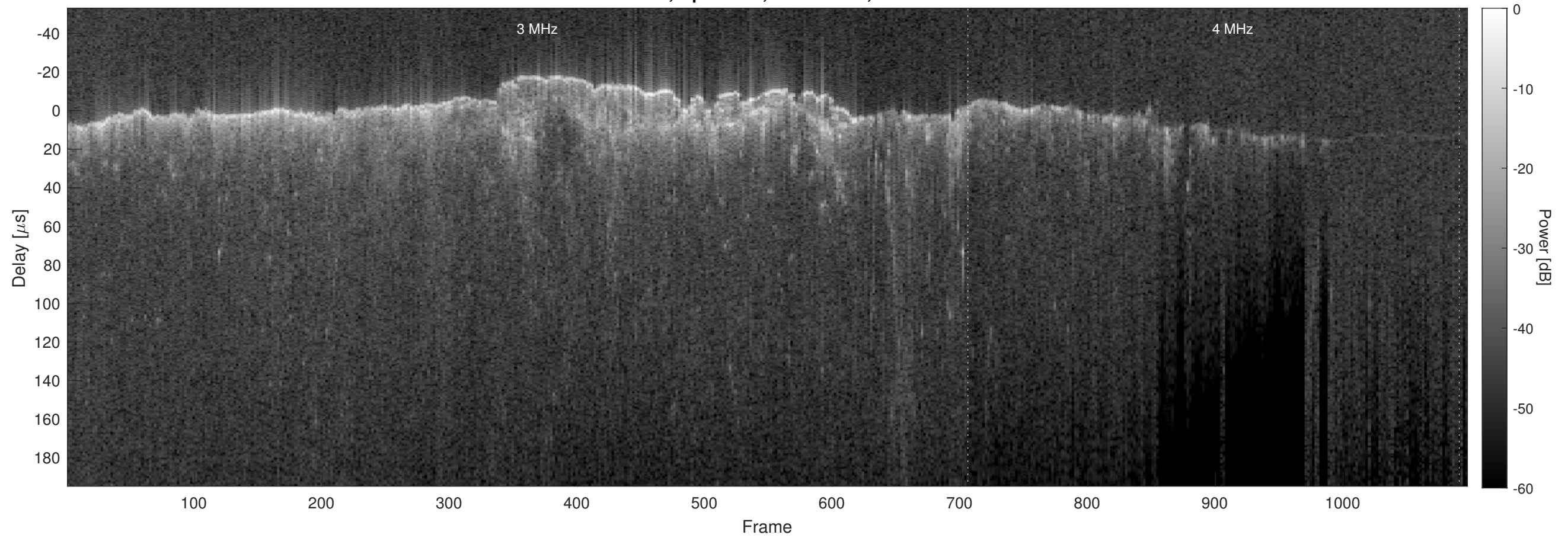
Orbit 12837, Optimized, No Window, Channel 2
