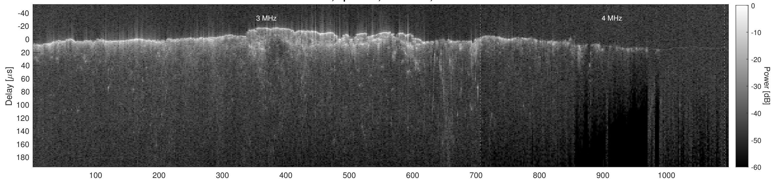
Orbit 12837, Cluttergram
