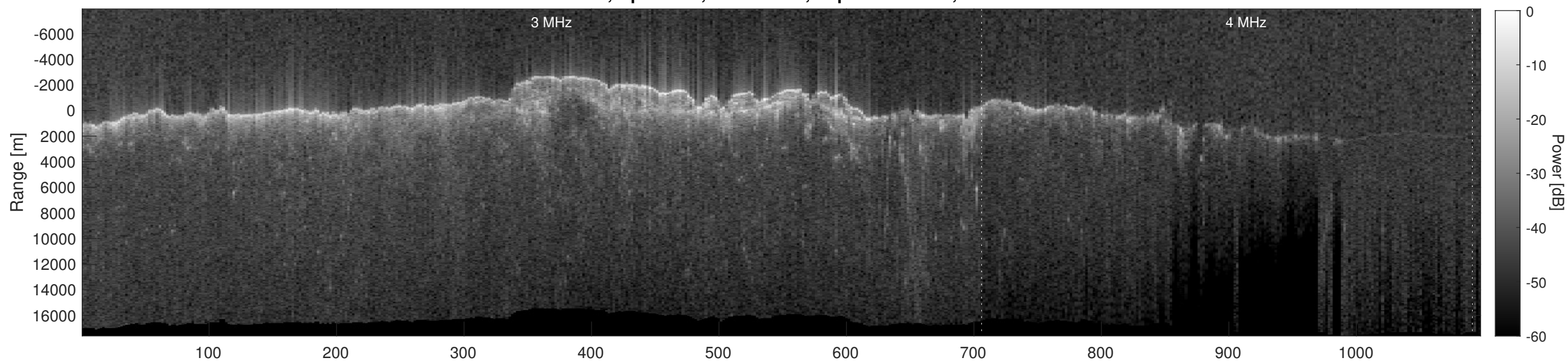
Orbit 12837, Depth-Corrected Cluttergram
