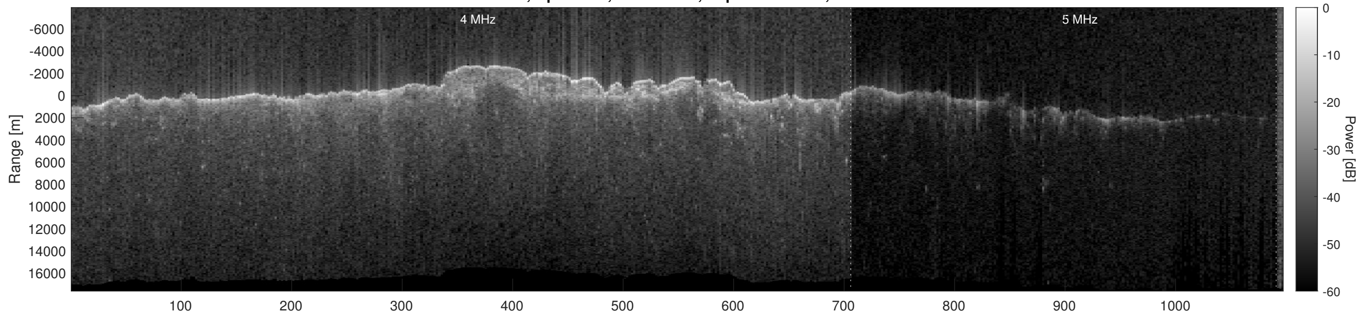
Orbit 12837, Optimized, No Window, Depth-Corrected, Channel 2
