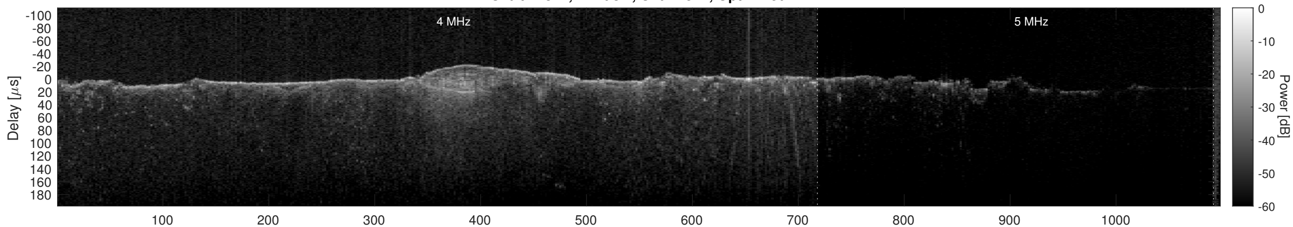
Orbit 12841, Cluttergram
