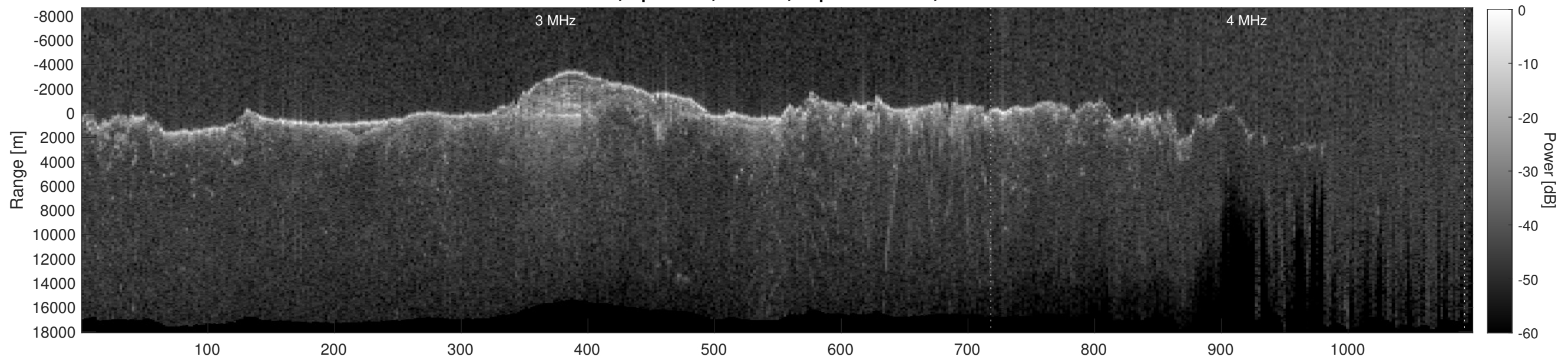
Orbit 12841, Depth-Corrected Cluttergram
