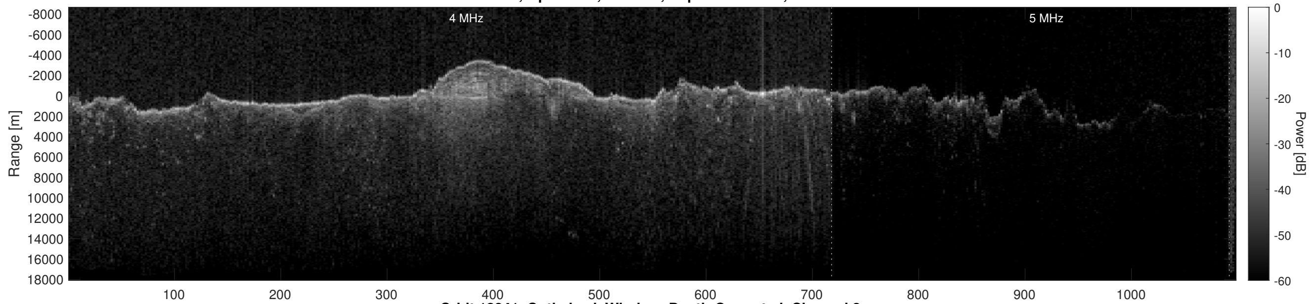
Orbit 12841, Optimized, Window, Depth-Corrected, Channel 2
