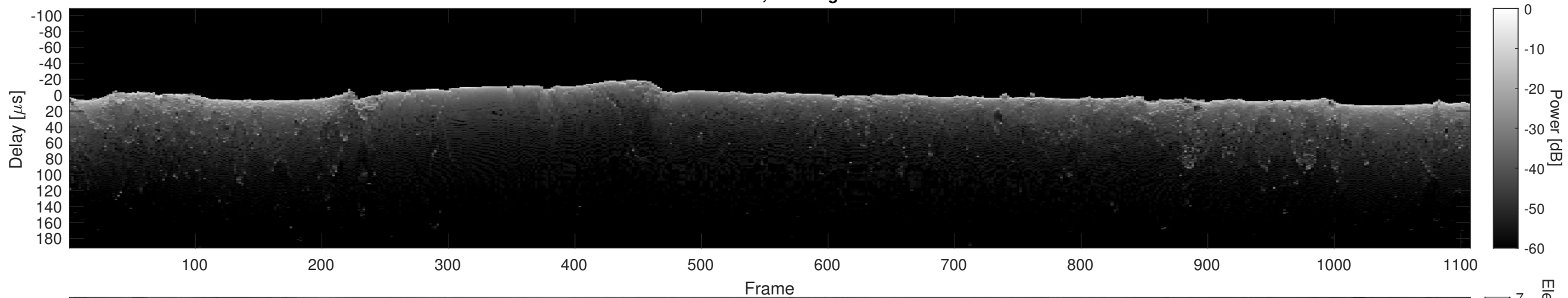
Orbit 12842, Cluttergram
