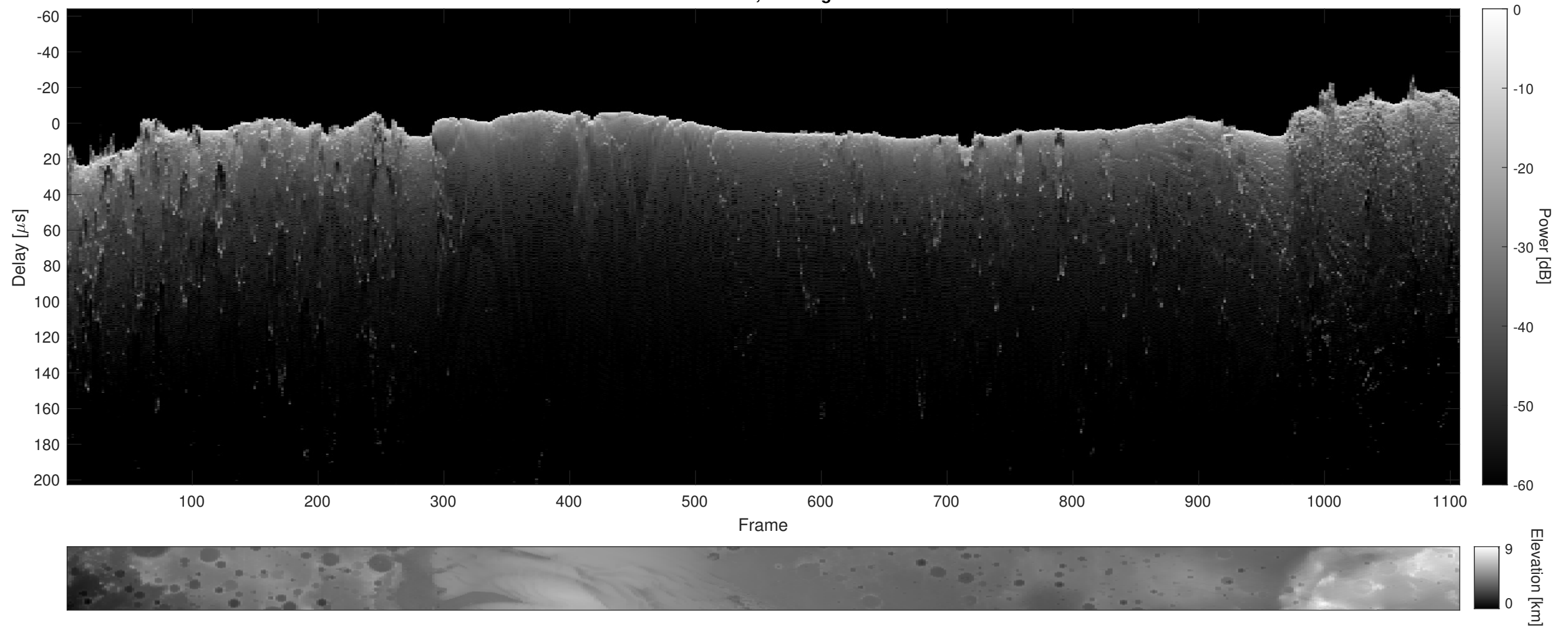
Orbit 12843, Cluttergram
