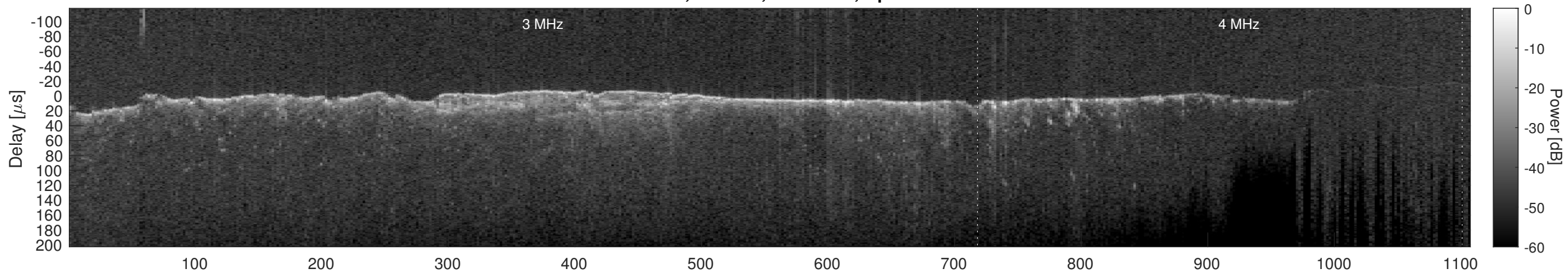
Orbit 12843, Cluttergram
