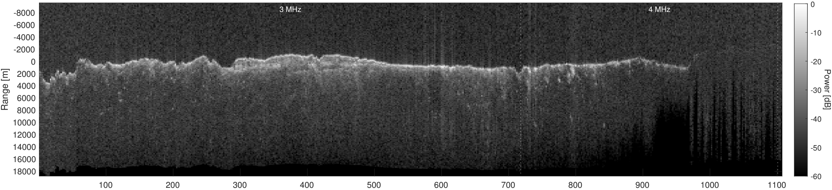
Orbit 12843, Depth-Corrected Cluttergram
