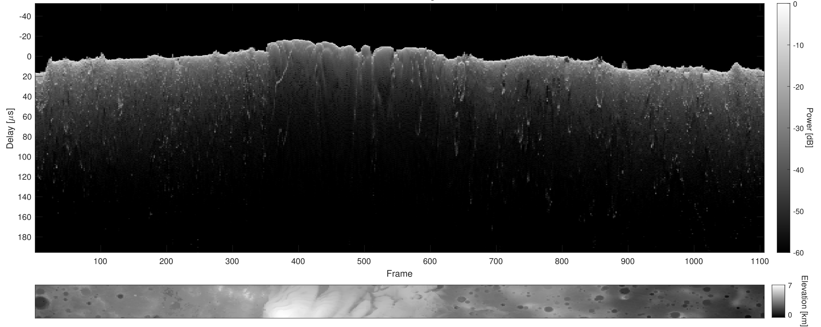
Orbit 12844, Cluttergram
