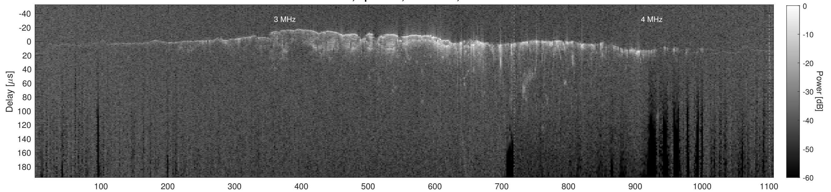
Orbit 12844, Cluttergram
