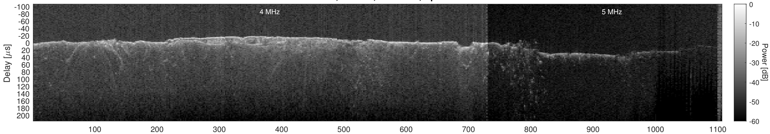
Orbit 12846, Cluttergram
