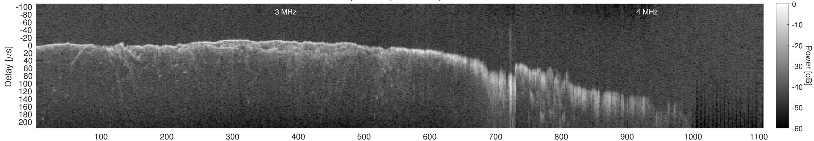
Orbit 12846, Window, Channel 2, Chapman
