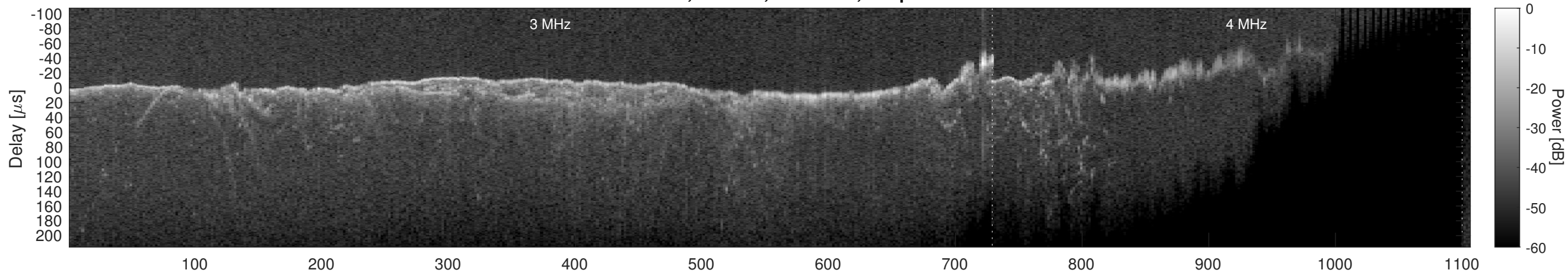
Orbit 12846, Window, Channel 2, Optimized
