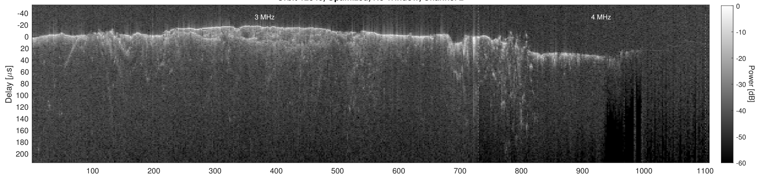
Orbit 12846, Cluttergram
