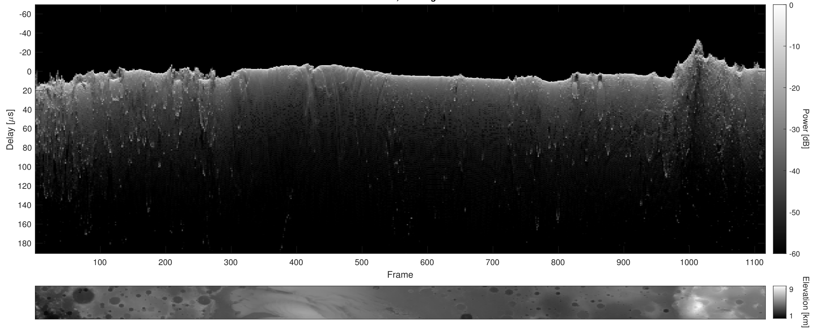
Orbit 12850, Cluttergram
