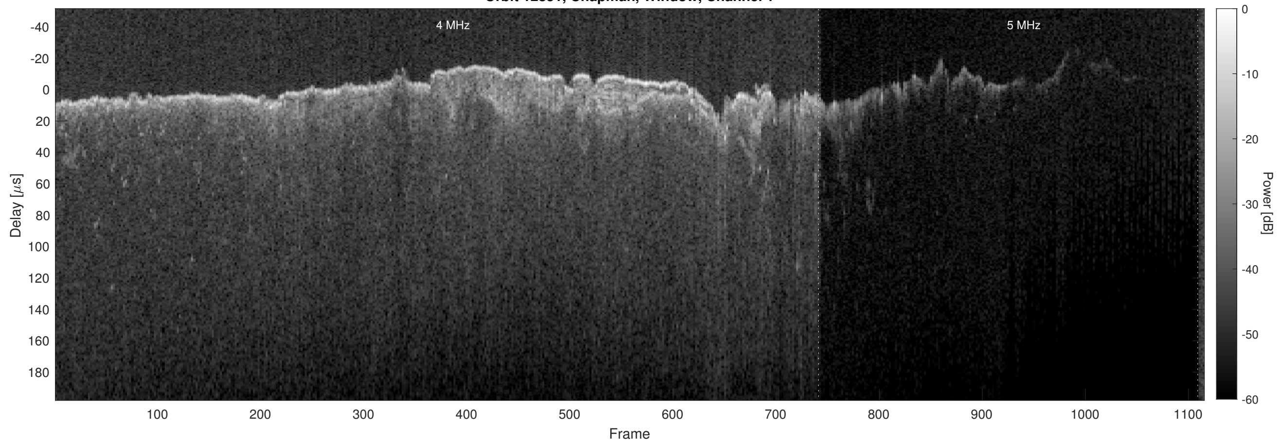
Orbit 12851, Chapman, Window, Channel 2
